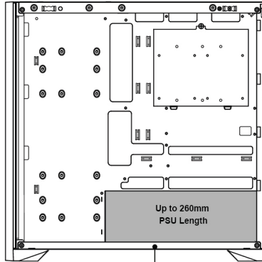
Power Supply Unit Installation
