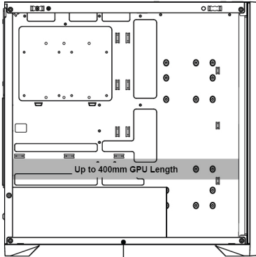
Graphics Processing Unit and other expansion cards
