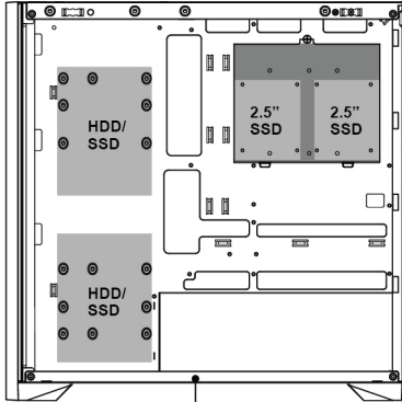
SSD Installation
