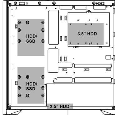
HDD Installation
